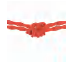
TLCB02002OG Ø 5.5 mm ∅ 2 x 0.75 mm 2 ‡ 1.5 / 3 / 15 / 30 / 50 m
